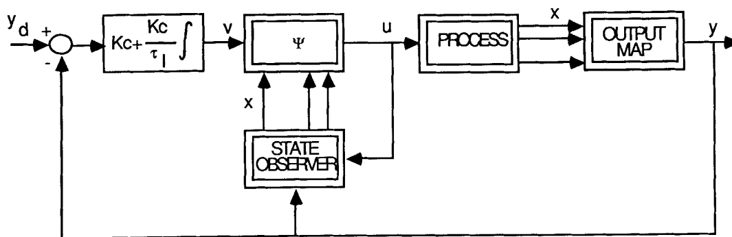
Figure 2. Globally linearizing control structure with a state observer.
